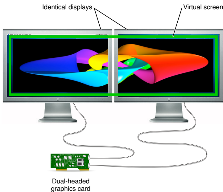
Figure 1-10 A virtual screen can represent more than one physical screen
