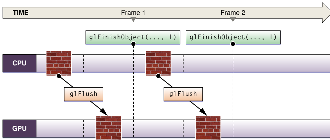
Figure 10-10 Single-buffered data
