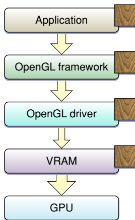
Figure 10-3 Data copies in an OpenGL program
