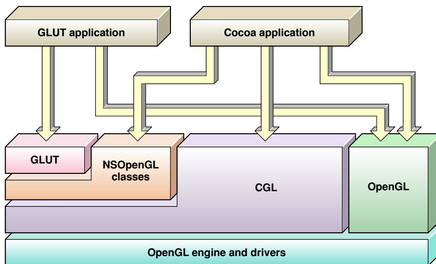
Figure 1-6 The programming interfaces used for OpenGL content
