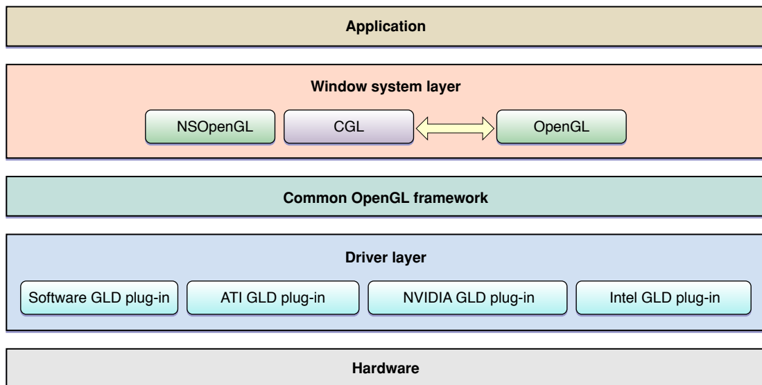
Figure 1-5 Layers of OpenGL for Mac OS X
