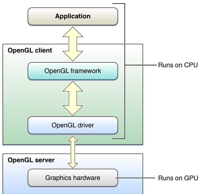
Figure 1-4 MacOS X OpenGL driver model
