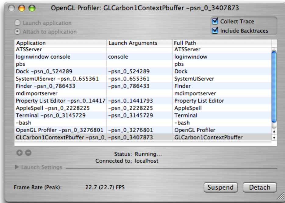
Figure 14-2 The OpenGL Profiler window
