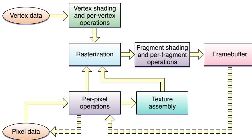
Figure 1-12 The flow of data through OpenGL
