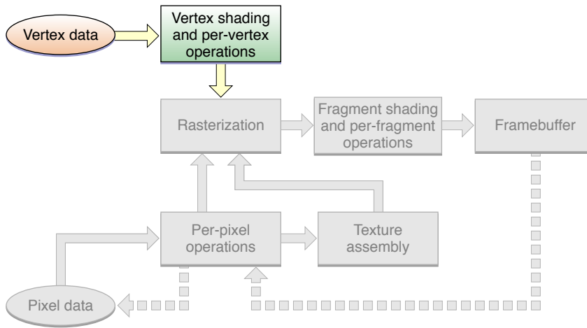
Figure 9-2 Vertex data path
