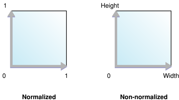
Figure 10-7 Normalized and non-normalized coordinates
