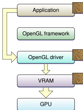
Figure 10-4 The client storage extension eliminates a data copy
