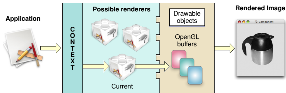
Figure 1-7 Data flow through OpenGL
