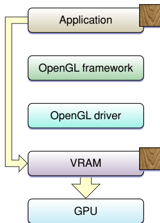
Figure 10-6 Combining extensions to eliminate data copies
