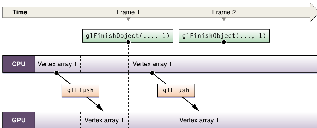
Figure 8-4 Single-buffered vertex array data
