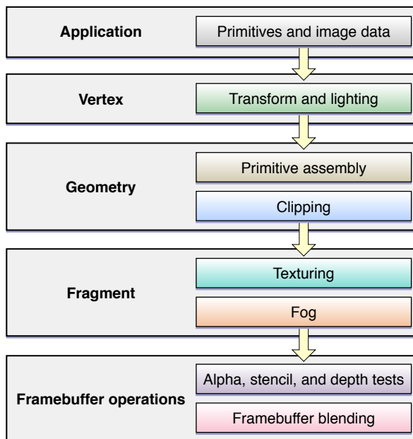
Figure 11-1 OpenGL fixed-function pipeline
