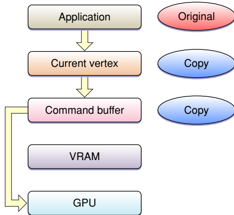
Figure 9-3 Immediate mode requires a copy of the current vertex data
