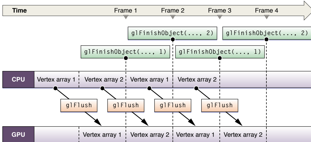
Figure 8-5 Double-buffered vertex array data
