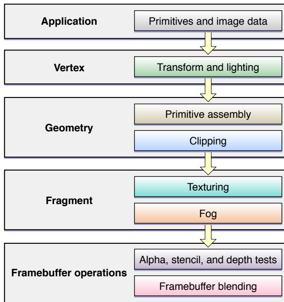
Figure 8-1 OpenGL graphics pipeline
