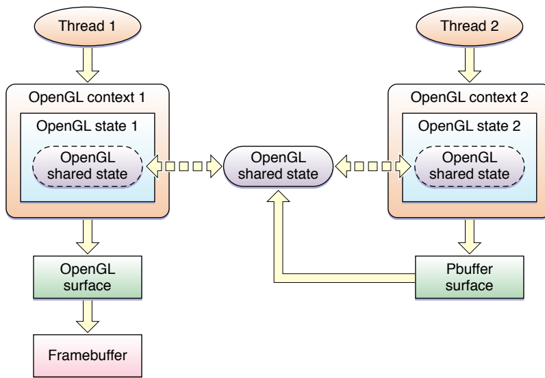
Figure 13-2 Two contexts on separate threads
