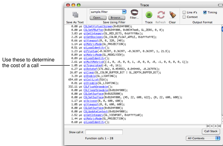
Figure 14-4 A Trace window
