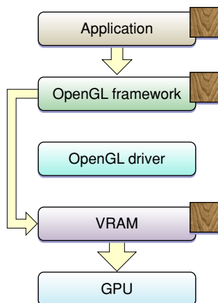
Figure 10-5 The texture range extension eliminates a data copy
