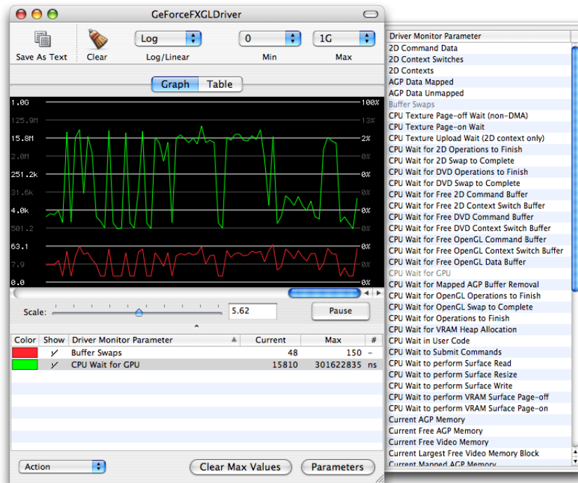
Figure 14-5 The graph view in OpenGL Driver Monitor
