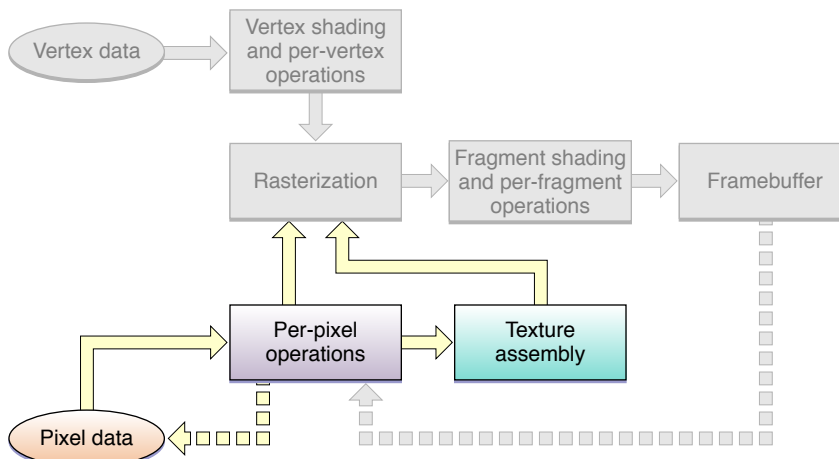
Figure 10-2 Texture data path
