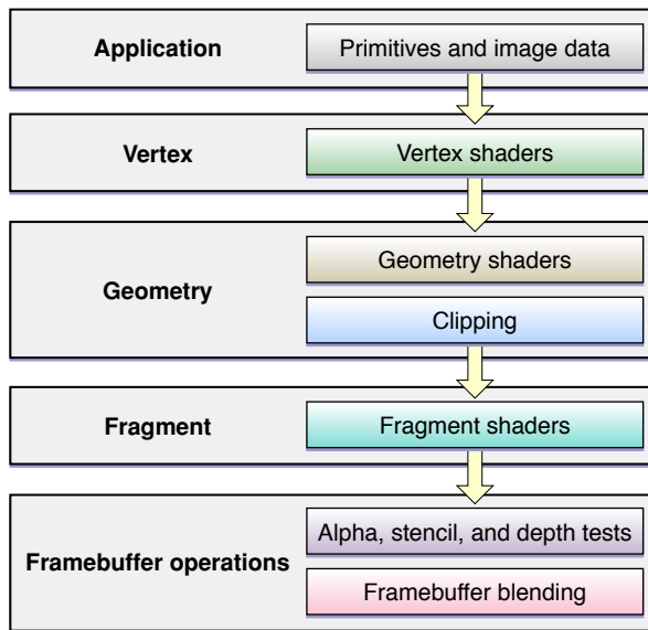
Figure 11-2 OpenGL shader pipeline
