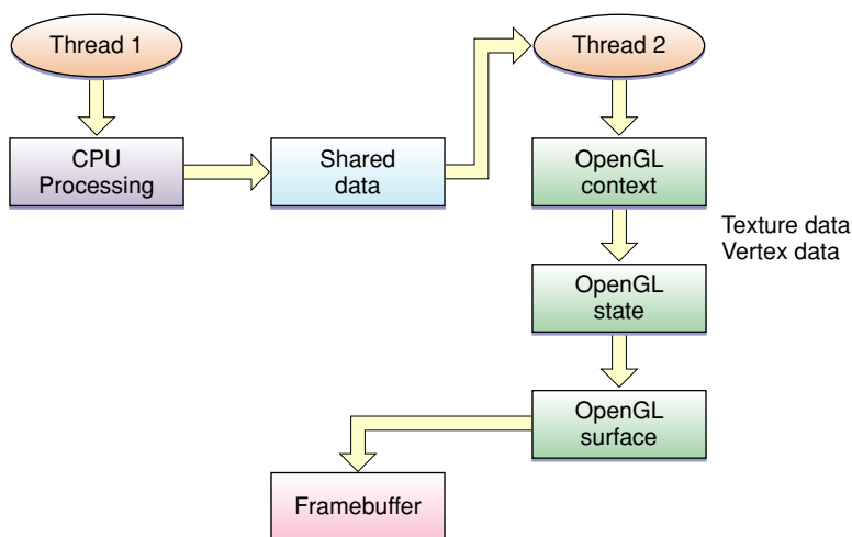
Figure 13-1 CPU processing and OpenGL on separate threads
