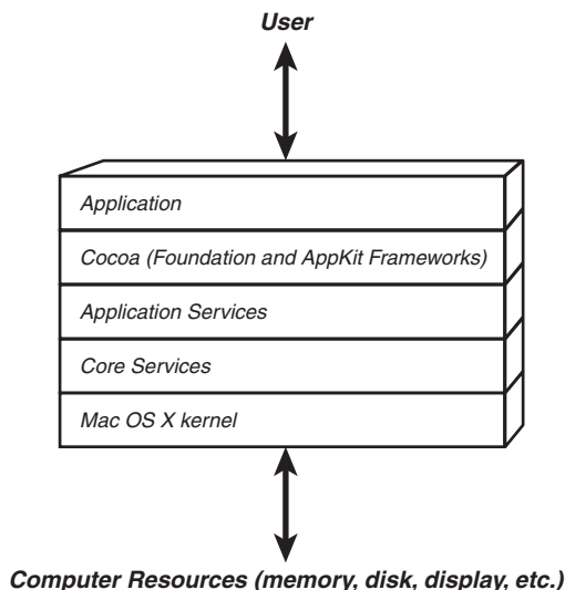
Figure 20.1 The application hierarchy
