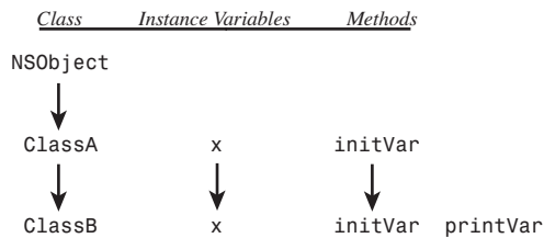
Figure 8.3 Inheriting instance variables and methods.
