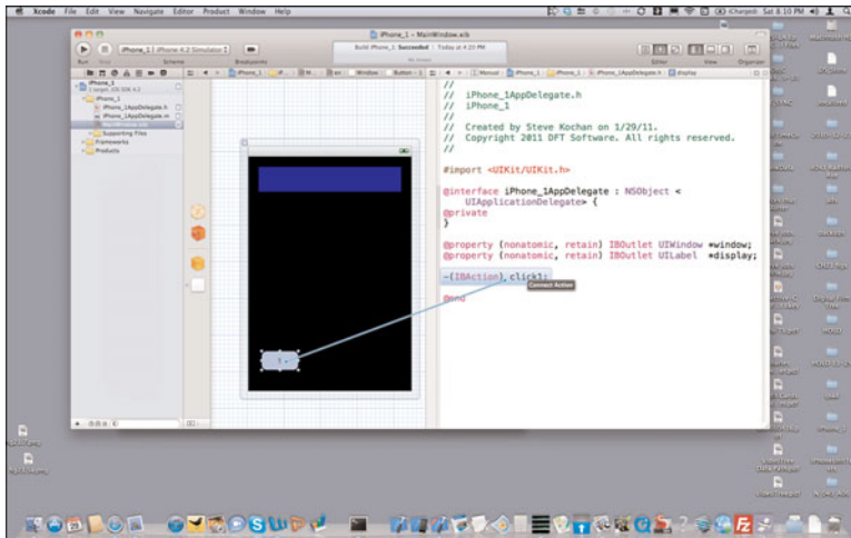
Figure 21.15 Adding an action for a button.
