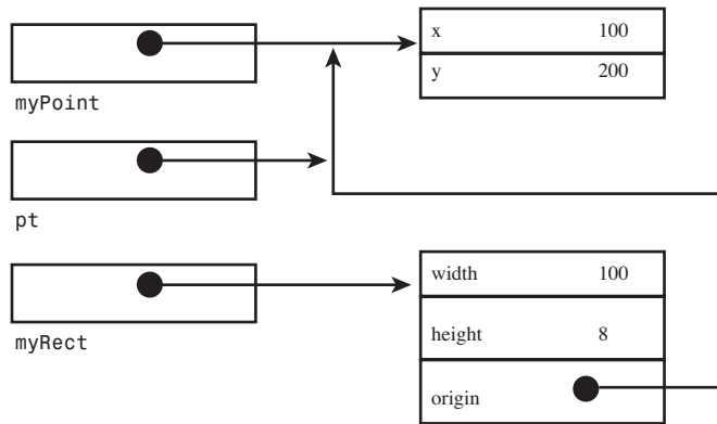
Figure 8.7 Setting the rectangle's origin
