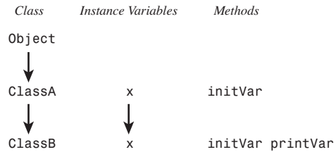
Figure 8.9 Overriding the initVar method
