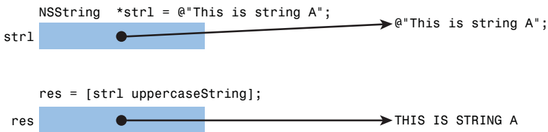
Figure 15.2 Sending the uppercaseString message to a string object
