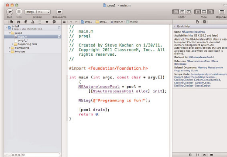
Figure 14.3 Quick Help displayed in the View pane.
