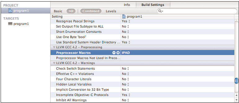
Figure 12.1 Defining the preprocessor identifier IPAD
