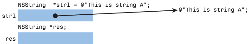
Figure 15.1 Immutable string object declaration and initialization
