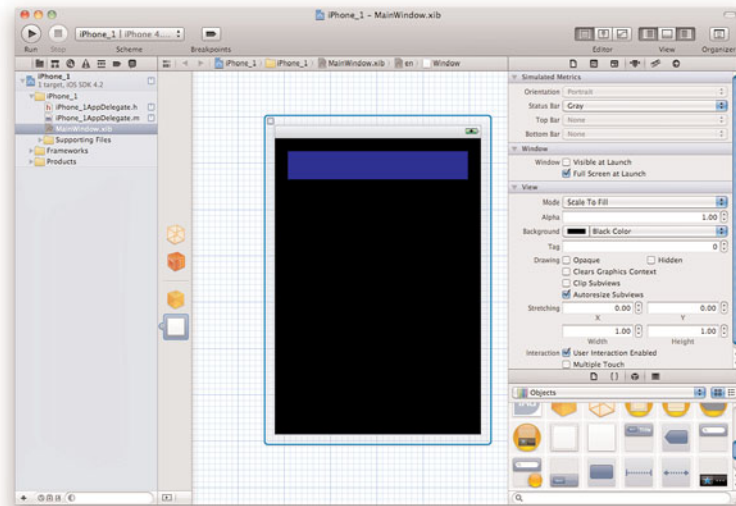
Figure 21.12 Changing the label's attributes and size.
