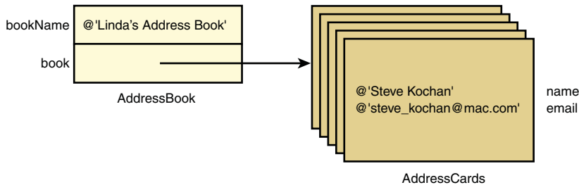
Figure 15.5 An AddressBook that contains AddressCards
